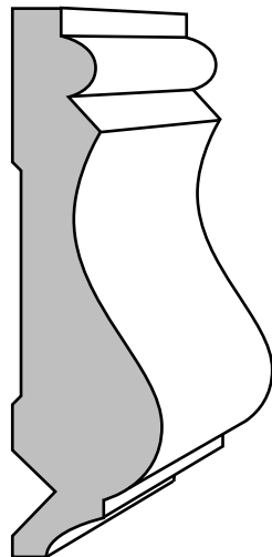
F720 11/16" X 2-5/8" OAK - POPLAR
