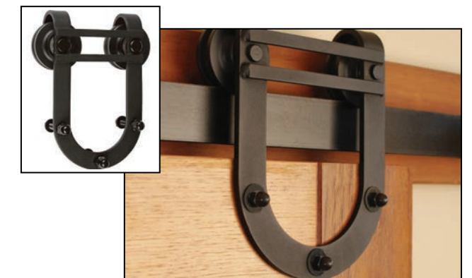
2000 SERIES (HORSESHOE) Available in: Black 330 lb. Limit Per Set
