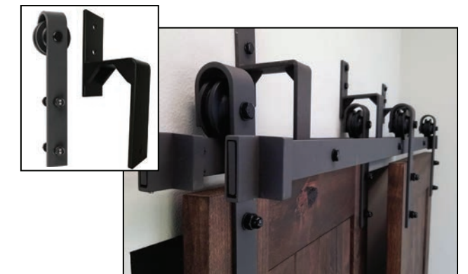
BYPASS KIT (STANDARD) Available in: Black only with 1000 series hangers 300 lb. Limit Per Set
