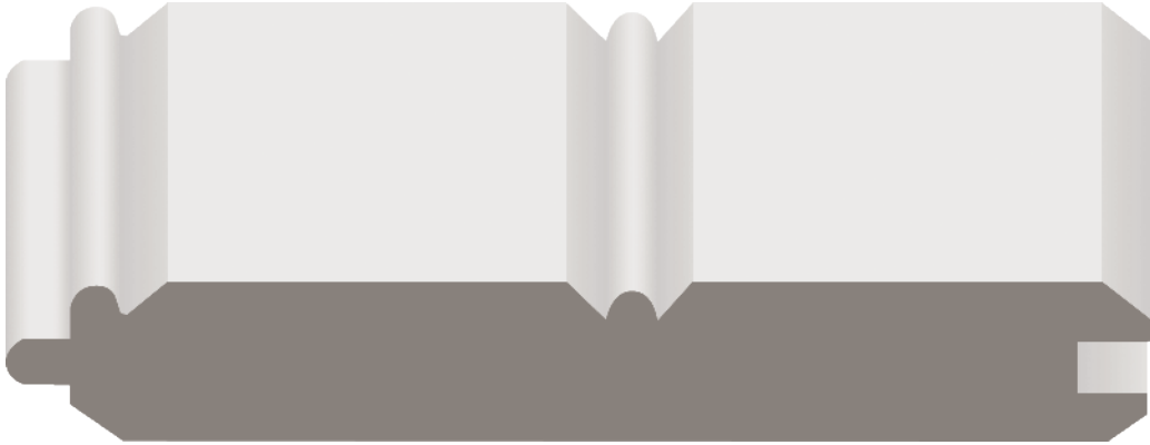
Stock Code 3454TVGP Dimensions 3/4" X 5 3/8" X 16' (1382736) PFJ
