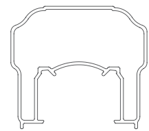
IMPRESSION RAIL EXPRESS® TOP RAIL SIZE: 2.5" X 2.3"
