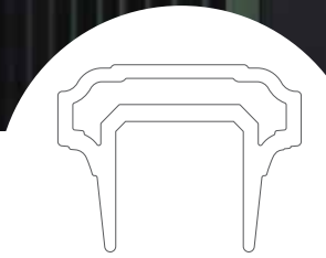
PREMIER RAILING® TOP RAIL SIZE: 3.5" X 2.7"
