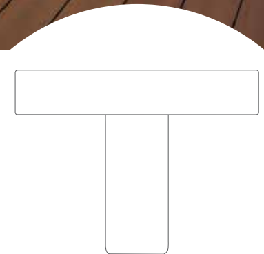
BUILDER RAIL TOP RAIL SIZE: 3.4" X 1.5"
