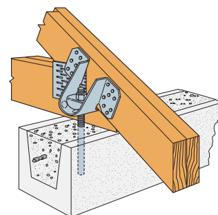
Typical VGT Installation
