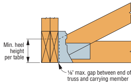
HTU Installation for Standard Allowable Loads (for 1 \frac{1}{2} " maximum gap, use Alternate Allowable Loads.)
