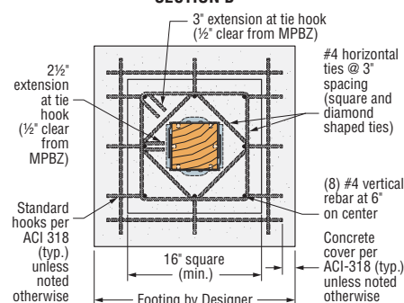
MPB66Z Reinforced Concrete Footing
