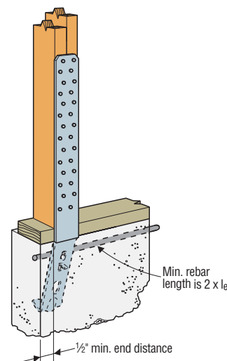
Typical STHD10 End-Wall Installation
