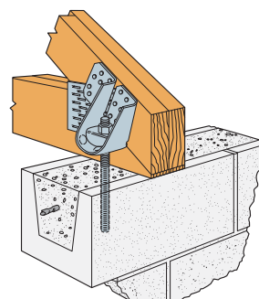
Typical VGTR Installation
