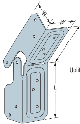
KBS1Z U.S. Patent 9,045,895
