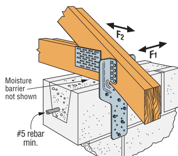
Typical LGT2 Installation into Masonry (LGT3 and LGT4 similar, but installed with Titen HD)
