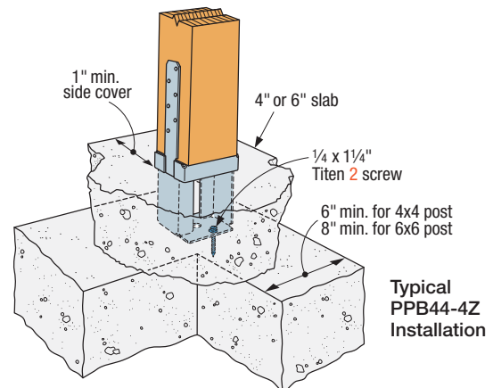
PPB44-4Z (other sizes similar)
