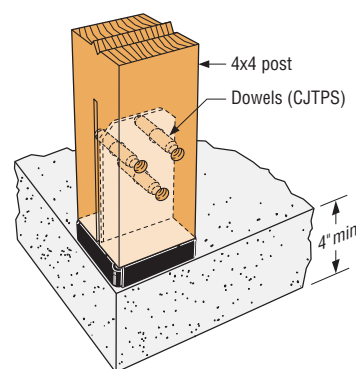
Typical CPT44Z Installation
