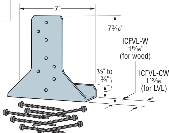
ICFVL-W and ICFVL-CW
