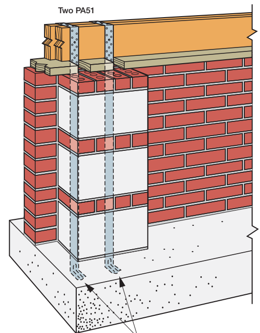
Minimum Two Straps per Pier Minimum 4" Embedment into Footing Per ICC 600-2014, Section 505.2.2.2., the assembly shown above is limited to 140 mph, SDC A and B, and one- and two-story buildings.
