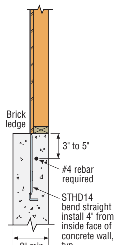
Brick-Ledge Installation without Step
