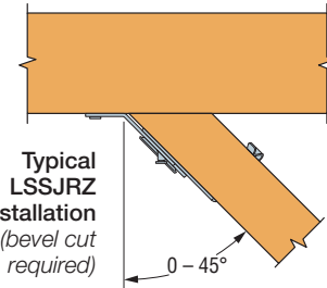
Typical LSSJLZ Installation (bevel cut required)
