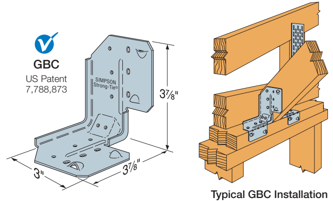
Typical GBC Installation
